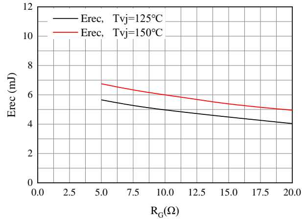
图 22. 开关损耗 二极管 Figure 22. Switching losses of Diode R_{gon} = 8\Omega, V_{CE} = 600V
